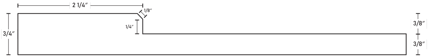
7007 3/8 V-Groove does not run through stile and rail joint
