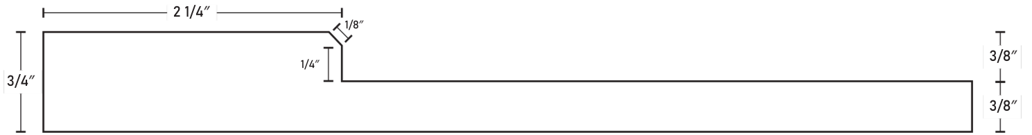
7005 3/8 V-Groove runs through stile and rail joint
