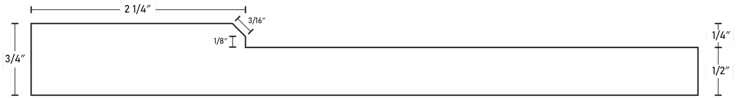
7005 V-Groove runs through stile and rail joint
